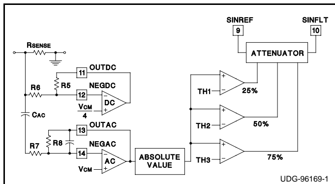
Figure 8. Current Limiting
