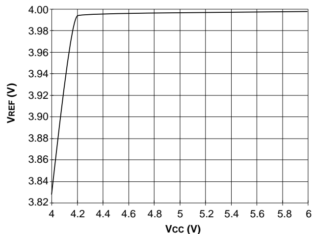
UCC1803/5 VREF vs. Vcc; LOAD = 0.5mA
