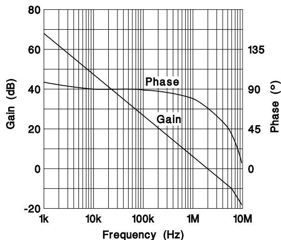
Error Amplifier Gain/Phase Response
