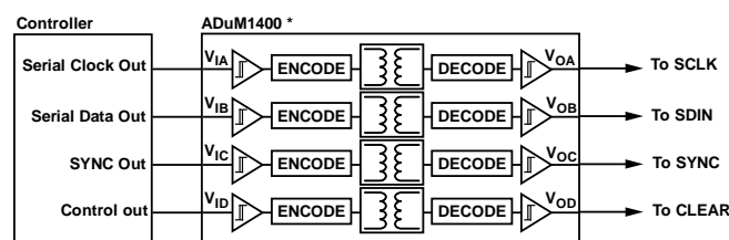
Figure 16. Isolated Interface
