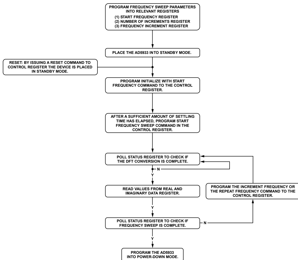
Figure 34. Frequency Sweep Flow Chart
