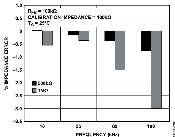
Figure 29. Impedance Range 4 Typical % Impedance Error over Frequency
