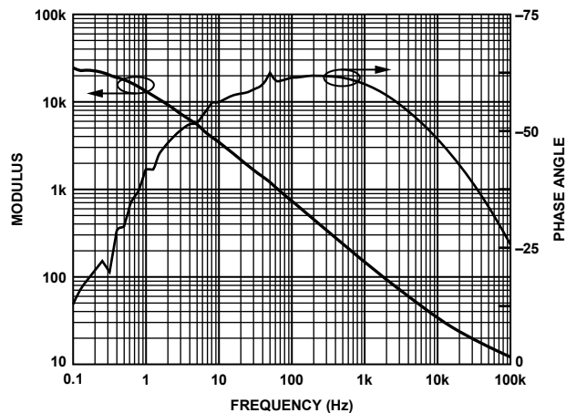
Figure 44. Bode Plot for Aluminum Corrosion Sensor
