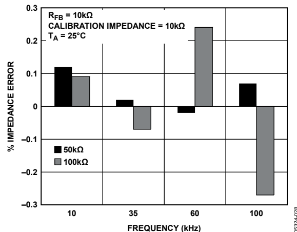
Figure 28. Impedance Range 3 Typical % Impedance Error over Frequency
