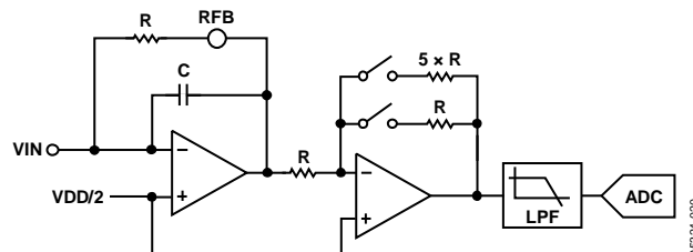
Figure 20. Receive Stage
