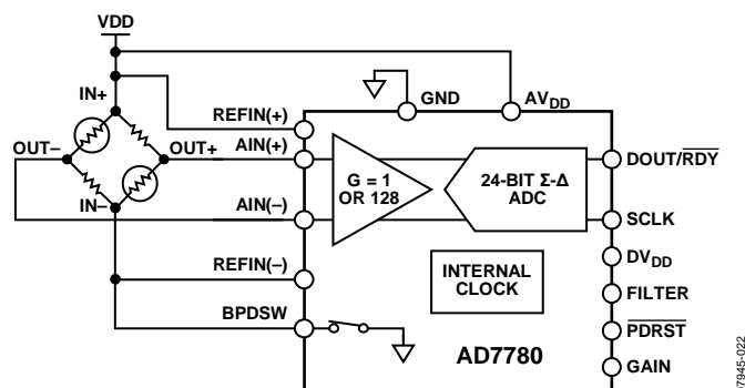
Figure 23. Weigh Scales Using the AD7780
