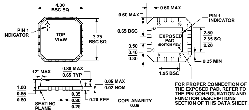
Figure 47. 16-Lead Lead Frame Chip Scale Package [LFCSP_VQ] 4 mm x 4 mm Very Thin Quad (CP-16-10)
