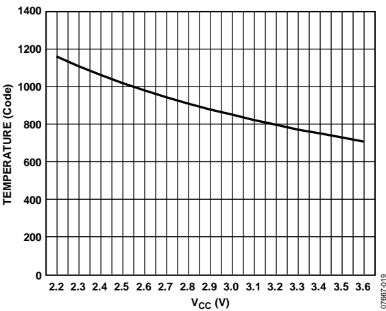
Figure 19. Temperature Code vs. V CC for 25°C
