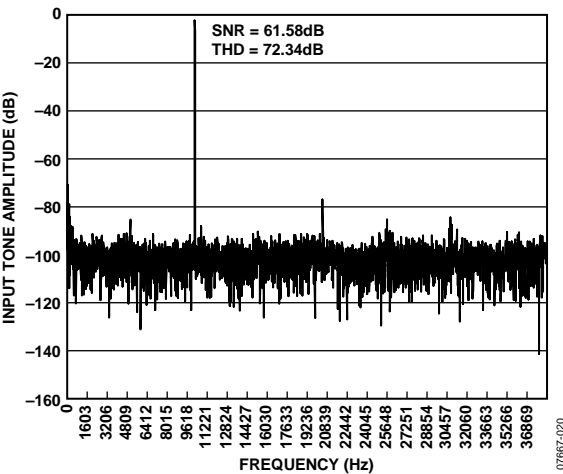
Figure 20. Typical FFT Plot for the Auxiliary Channels at 25 kHz Sampling Rate and 1 kHz Input Frequency
