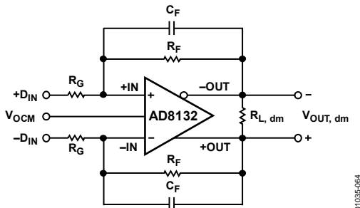
Figure 64. Circuit Definitions (Should V_{O, dm} be V_{OUT, dm} in the fig?)
