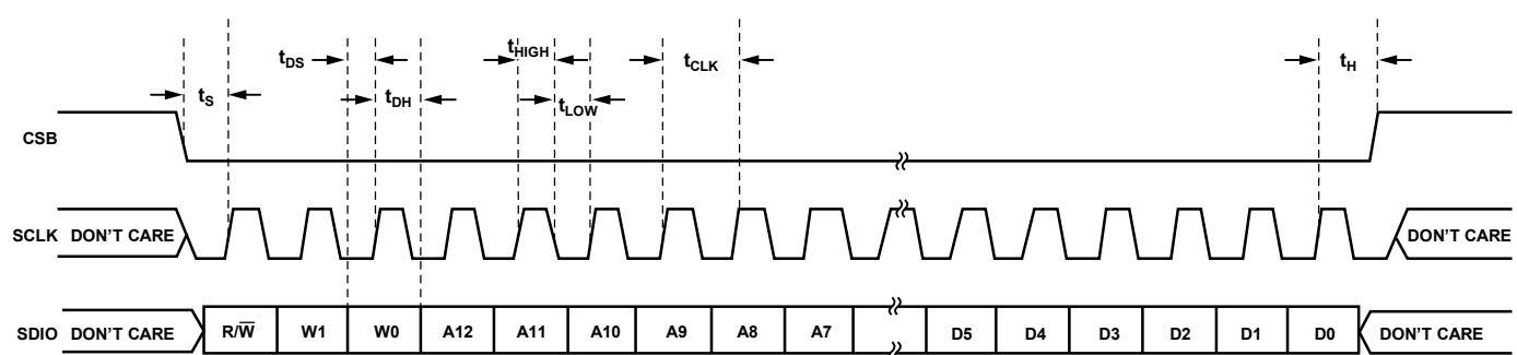
Figure 57. Serial Port Interface Timing Diagram
