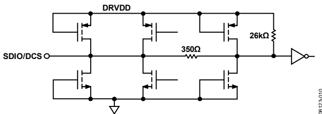
Figure 33. Equivalent SDIO/DCS Circuit
