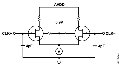
Figure 49. Equivalent Clock Input Circuit
