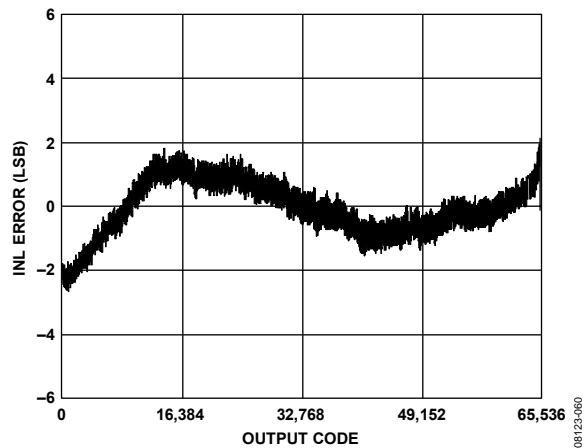
Figure 27. INL with f_{IN} = 9.7 MHz and Dither Enabled
