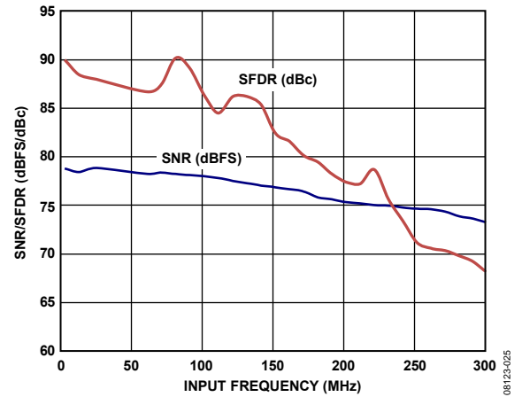
Figure 18. Single-Tone SNR/SFDR vs. Input Frequency ( f_{IN} ) with 2 V p-p Full Scale
