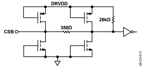
Figure 36. Equivalent CSB Input Circuit
