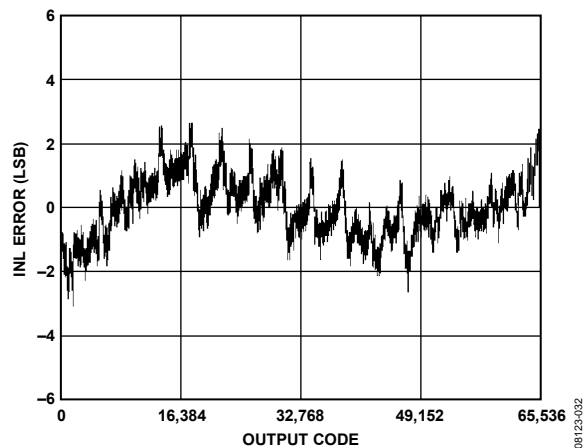
Figure 26. INL with f_{IN} = 9.7 MHz
