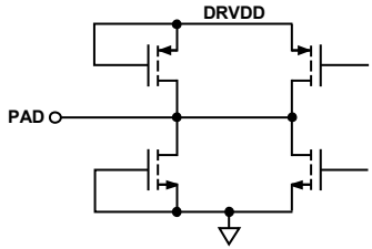
Figure 32. Digital Output
