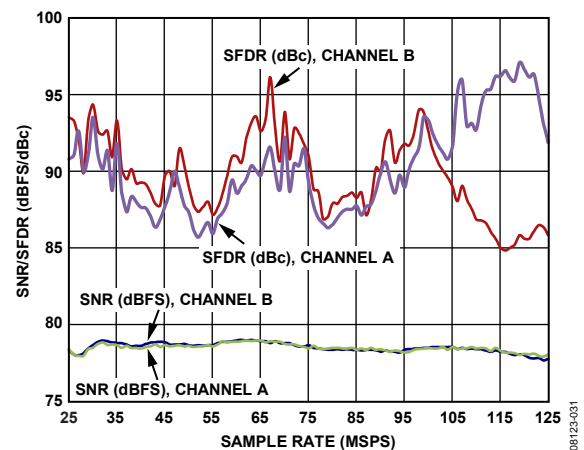
Figure 24. Single-Tone SNR/SFDR vs. Sample Rate ( f_s ) with f_{IN} = 70.1 MHz
