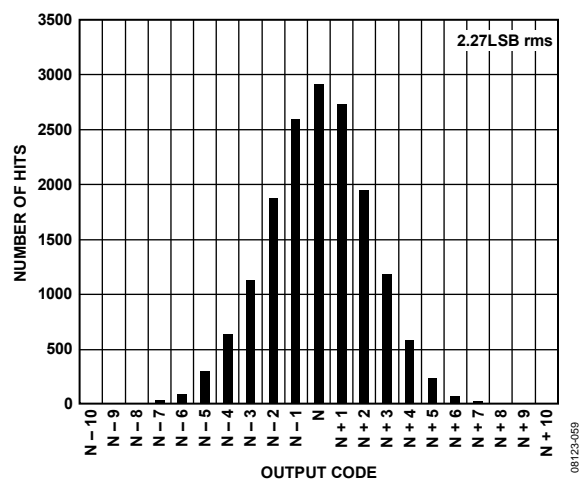
Figure 25. Grounded Input Histogram
