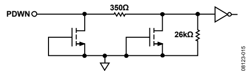
Figure 38. Equivalent PDWN Input Circuit
