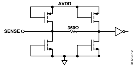
Figure 35. Equivalent SENSE Circuit
