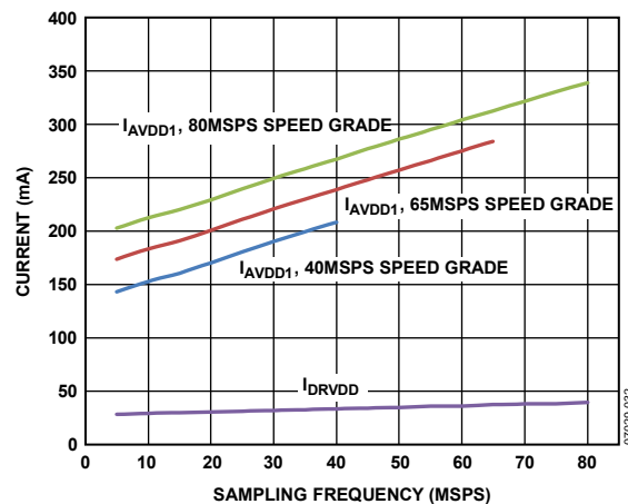
Figure 60. Supply Current vs. f_{\text{SAMPLE}} for f_{\text{IN}} = 5 \text{ MHz}
