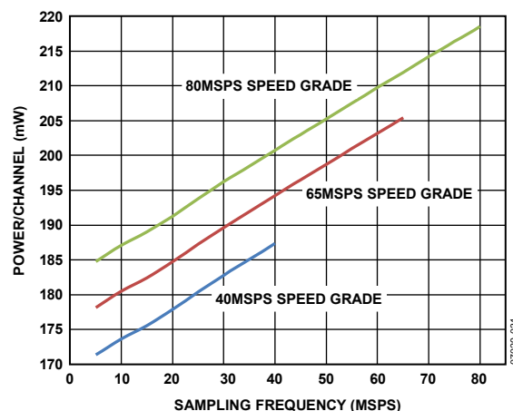
Figure 61. Power per Channel vs. f_{\text{SAMPLE}} for f_{\text{IN}} = 5 \text{ MHz}
