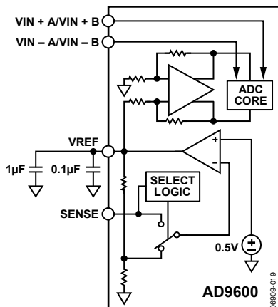
Figure 51. Internal Reference Configuration
