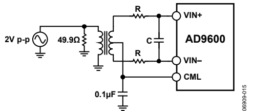
Figure 47. Differential Transformer-Coupled Configuration
