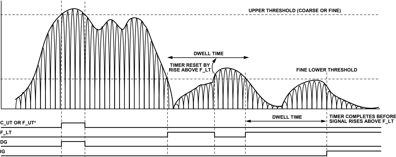
Figure 66. Threshold Settings for C_UT, F_UT, F_LT, IG, and DG
