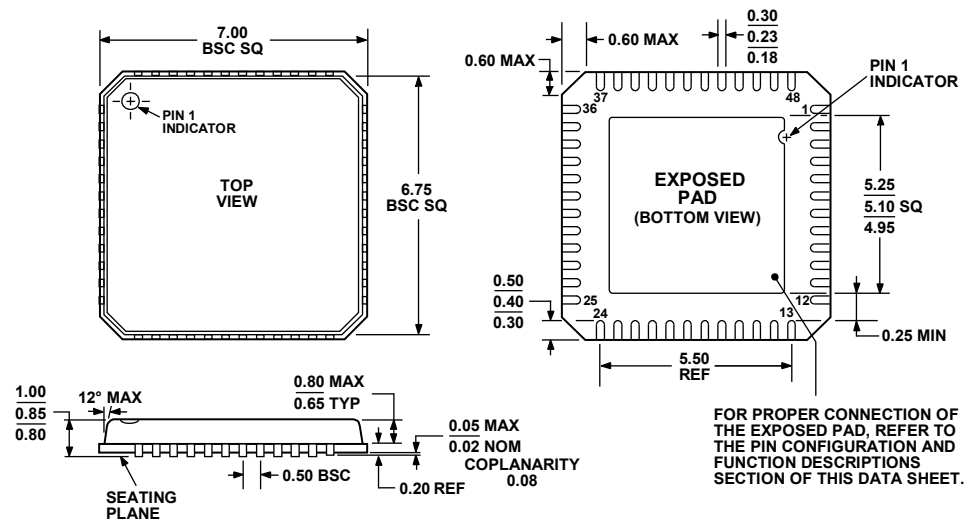
COMPLIANT TO JEDEC STANDARDS MO-220-VKKD-2 Figure 60. 48-Lead Lead Frame Chip Scale Package [LFCSP_VQ] 7 mm x 7 mm Body, Very Thin Quad (CP-48-1) Dimensions shown in millimeters
