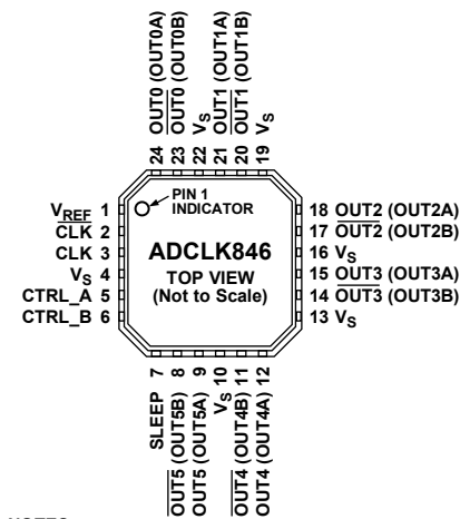
Figure 2. Pin Configuration
