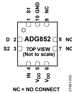
Figure 2. Pin Configurations
