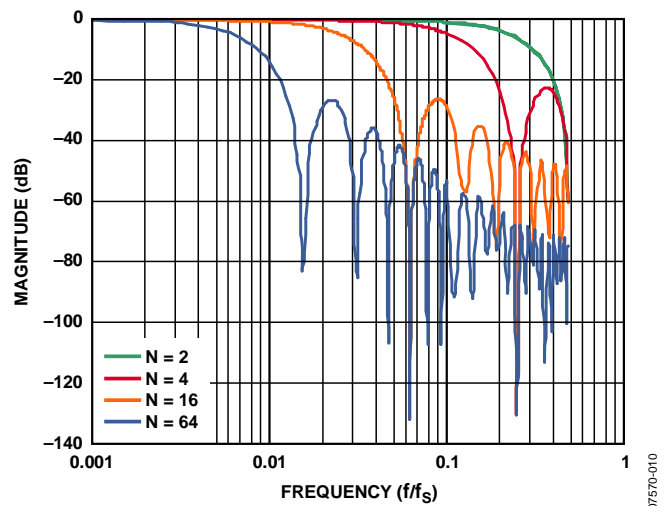
Figure 15. Bartlett Window FIR Frequency Response (Phase = M Samples)
