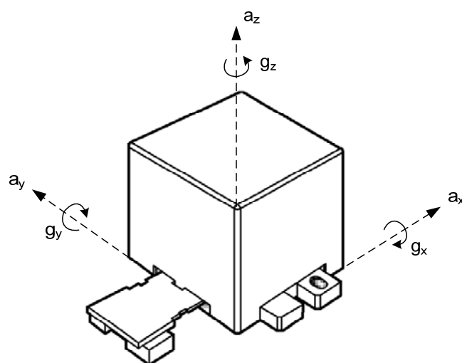
Figure 6. Axial Orientation
