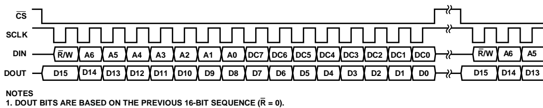
Figure 11. Output Register Bit Assignments
