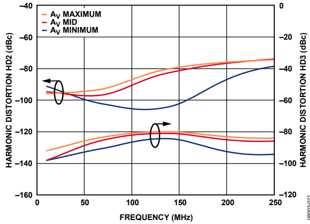
Figure 15. Harmonic Distortion vs. Frequency at A_V = 6 dB, 12 dB, and 15.5 dB, Output Level at 2 V p-p, R_L = 200\ \Omega
