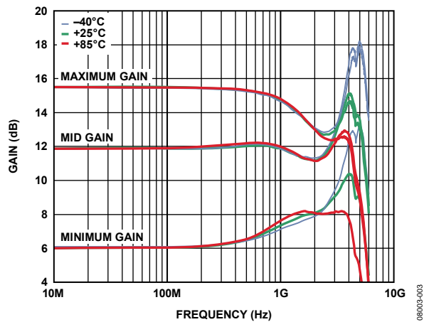
Figure 4. Gain vs. Frequency Response for 1 k \Omega Differential Load, A_V = 6\text{ dB} , 12 dB, and 15.5 dB over Temperature
