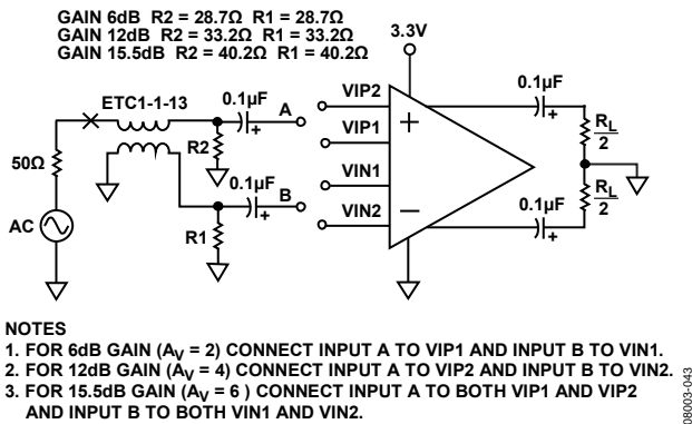
Figure 32. Differential-Input to Differential-Output Configuration
