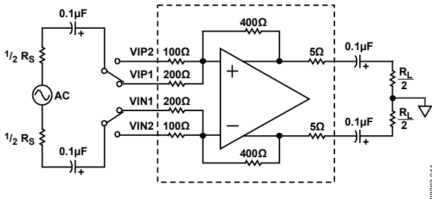
Figure 33. Differential Input Loading Circuit
