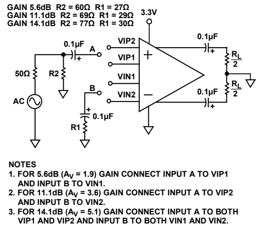
Figure 34. Single-Ended Input to Differential Output Configuration
