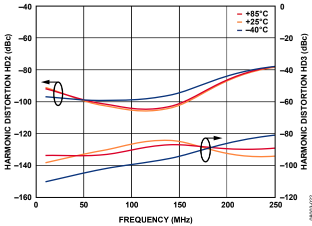
Figure 16. Harmonic Distortion vs. Frequency, Three Temperatures, Output Level at 2 V p-p, R_L = 200\ \Omega
