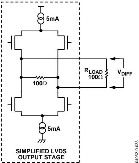
Figure 4. Differential Output Stage
