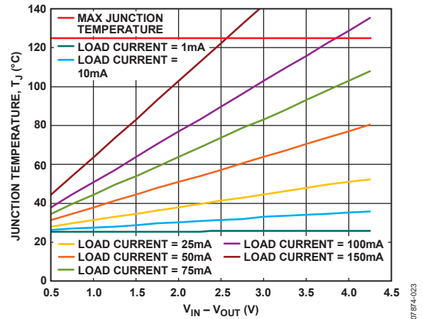
Figure 23. WLCSP, 0 mm² of PCB Copper, T_A = 25^\circ\text{C}
