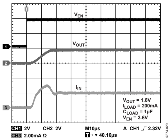
Figure 18. Typical Rise Time and Inrush Current with C_{LOAD} = 1 \mu F
