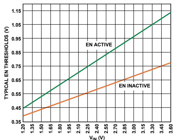
Figure 16. Typical EN Pin Thresholds vs. Input Voltage, V_{IN}
