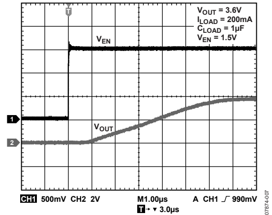
Figure 7. Turn-On Delay vs. Input Voltage = 3.6 V
