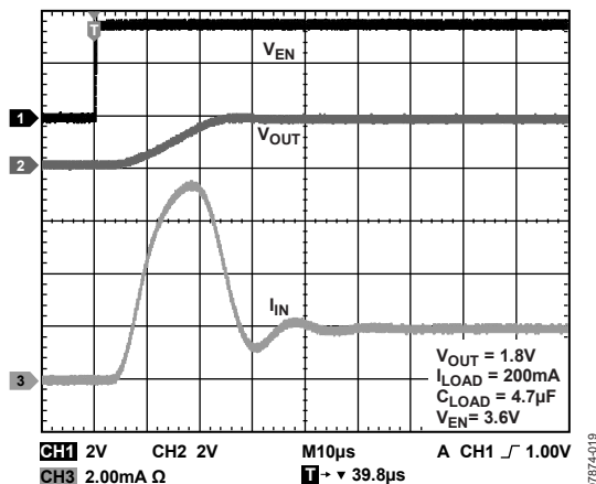
Figure 19. Typical Rise Time and Inrush Current with C_{LOAD} = 4.7 \mu F
