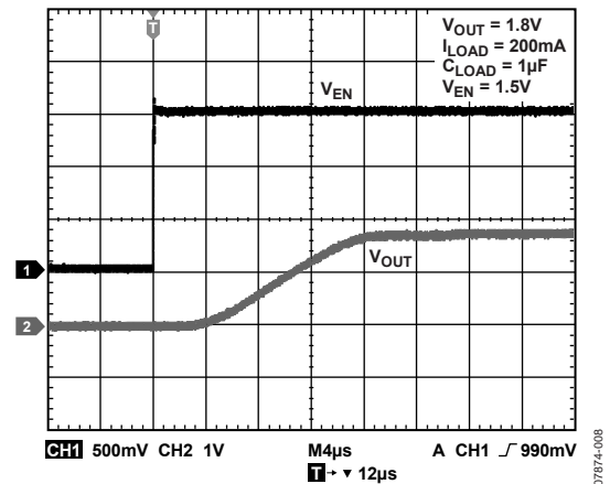
Figure 8. Turn-On Delay vs. Input Voltage = 1.8 V
