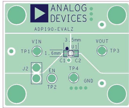
Figure 28. WLCSP PCB Layout
