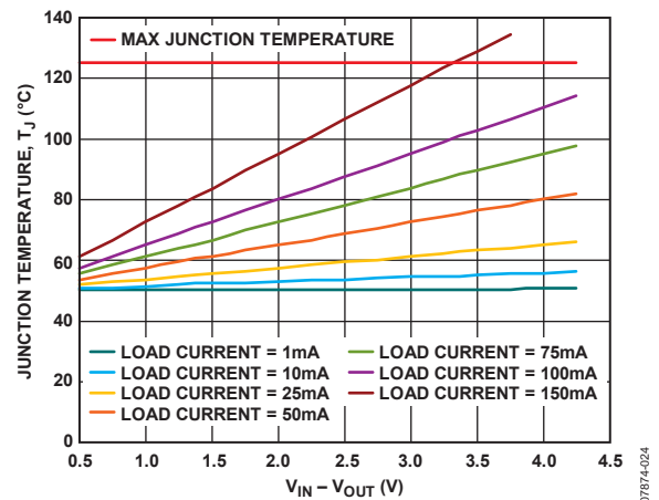
Figure 24. WLCSP, 500 mm² of PCB Copper, T_A = 50^\circ\text{C}
