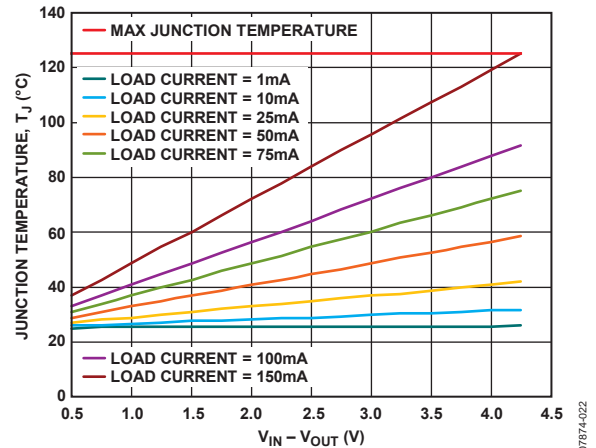
Figure 22. WLCSP, 100 mm² of PCB Copper, T_A = 25^\circ\text{C}
