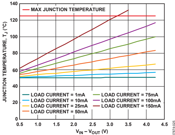
Figure 25. WLCSP, 100 mm² of PCB Copper, T_A = 50^\circ\text{C}
