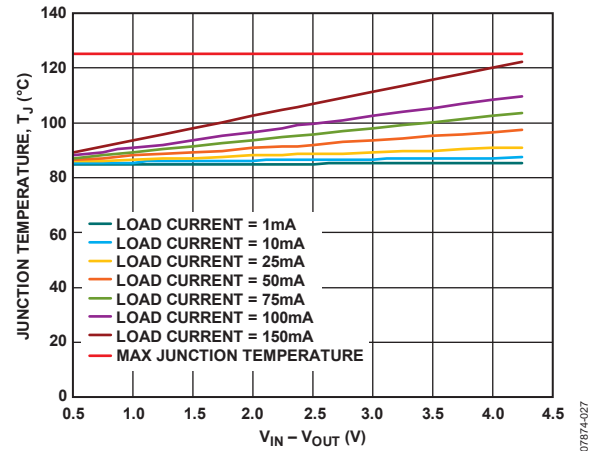
Figure 27. WLCSP, T_B = 85^\circ\text{C}
