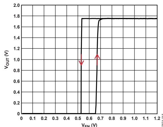
Figure 15. Typical EN Operation
