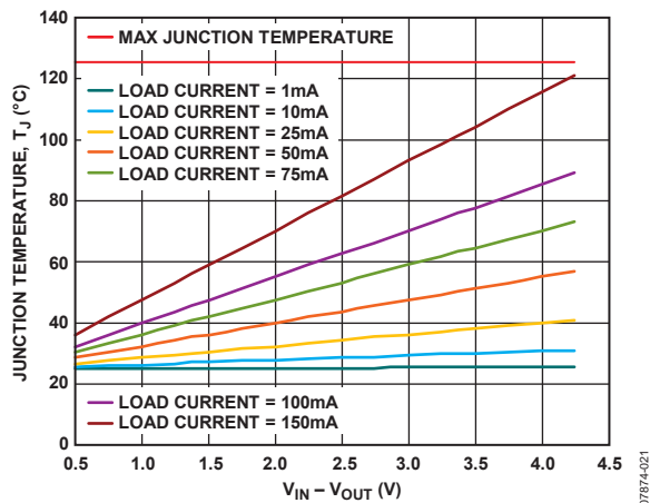
Figure 21. WLCSP, 500 mm² of PCB Copper, T_A = 25^\circ\text{C}
