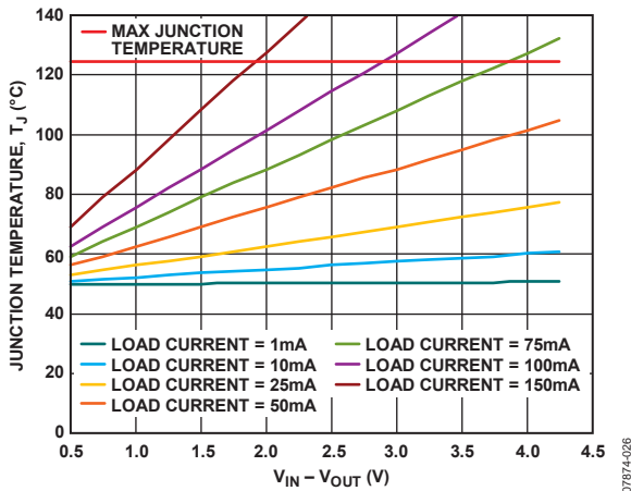
Figure 26. WLCSP, 0 mm² of PCB Copper, T_A = 50^\circ\text{C}
