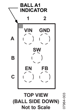
Figure 2. Pin Configuration
