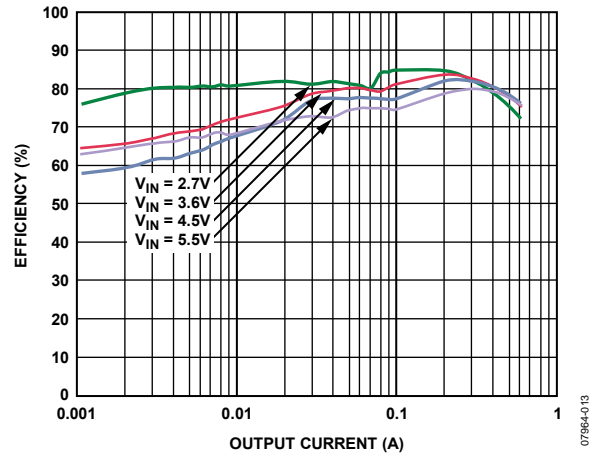
Figure 12. Efficiency, V_{OUT} = 1.0\text{ V}
