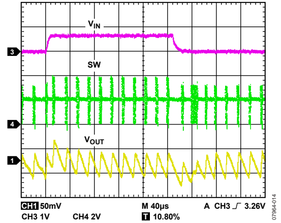
Figure 13. Line Transient, V_{OUT} = 1.8\text{ V} , Power Save Mode, I_{LOAD} = 20\text{ mA}
